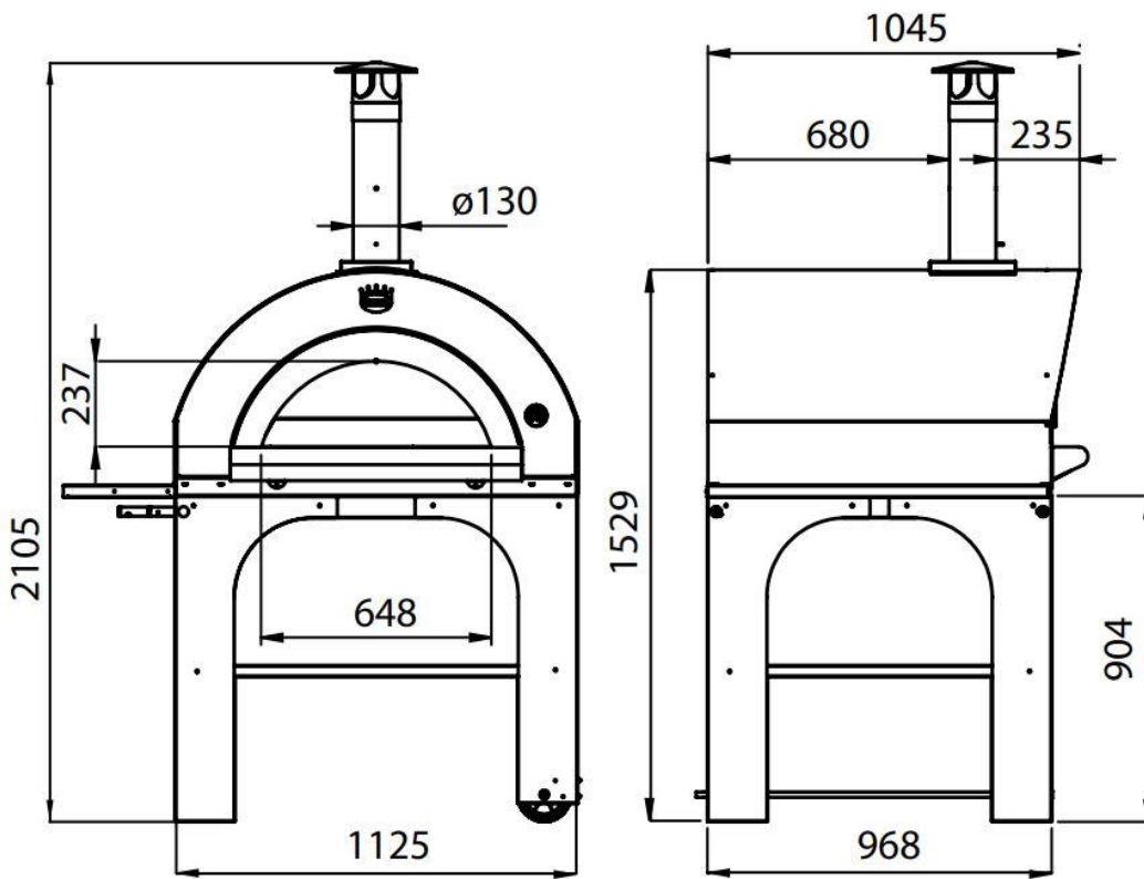
PULCINELLA 100x80 cm - kg 275
