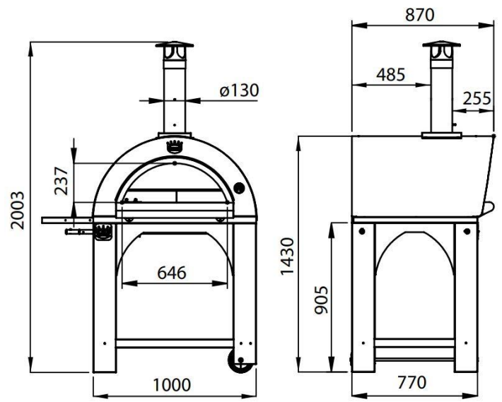
PULCINELLA 80x60 cm - kg 157
