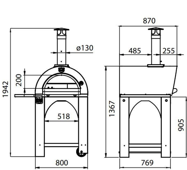
PULCINELLA 60x60 cm - Kg 130
